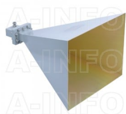
LB-229-20-C-NF Standard Gain Horn Antenna 3.3-4.9GHz 20dB Gain N Type Female
